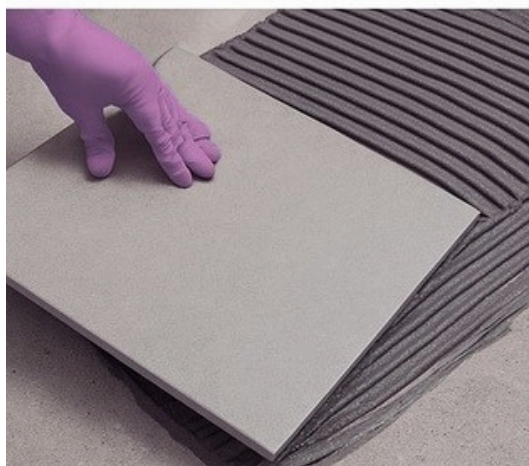
3. Tile Fixing
